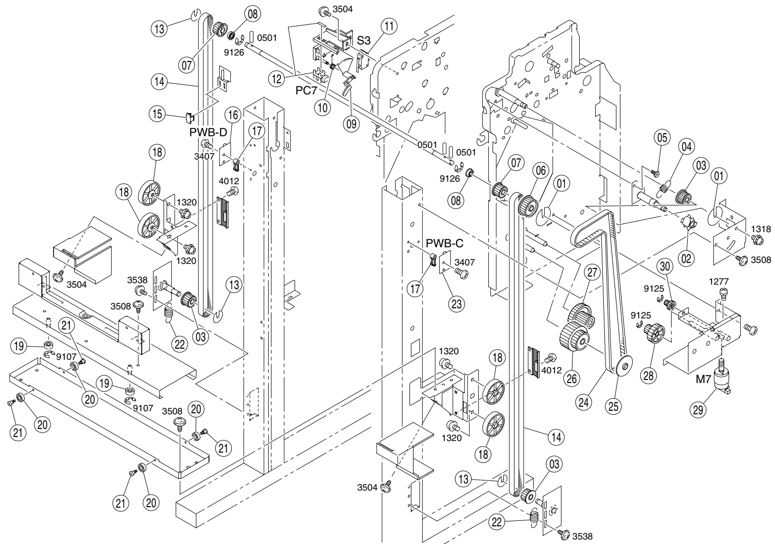
FIG. 4 ELEVATOR DRIVE
